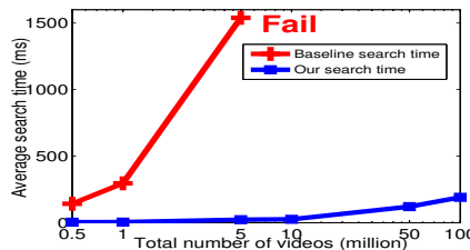
(b) Search Time (in ms)
